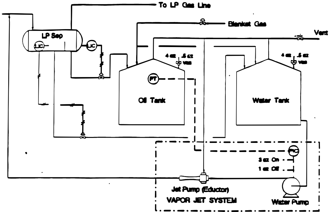
Figure 1 Schematic – Vapor Jet Vapor Recovery System
